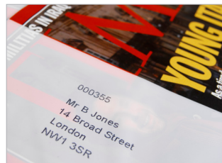
Addressing application on poly wrap printed from a Domino Bitjet+ ink jet printer
